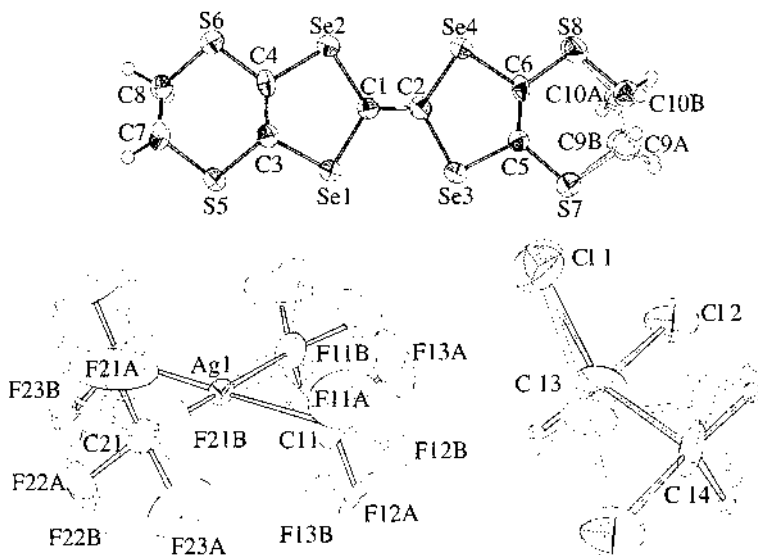
Fig. 11. Atomic numbering scheme for the \kappa_L\text{-(BEDT-TSF)}_2\text{Ag}(\text{CF}_3)_4(\text{TCE}) structure.
