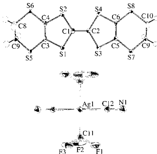
Fig. 10. Atomic numbering scheme for the (\text{ET})_2\text{Ag}(\text{CF}_3)_2(\text{CN})_2 structure.
