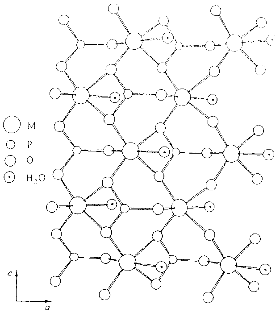
Fig. 4. The 4-connected net in the basal plane of (\text{RPO}_3)_\text{M} \cdot \text{H}_2\text{O} [13].
