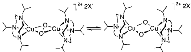
Fig. 7. Equilibrium between (\mu\text{-}\eta^2\text{:}\eta^2\text{-peroxo}) dicopper(II) and bis (\mu\text{-oxo}) dicopper(III) complexes that is shifted to the right by selective precipitation/aggregation of the latter under certain conditions (e.g. \text{X} = \text{ClO}_4^- , THF solvent).
