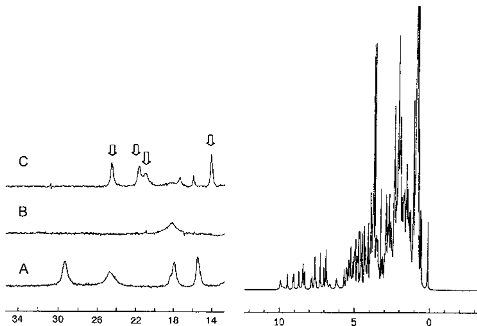
Fig. 2. ^1\text{H} -NMR spectra of D. gigas FdII. (A) Full spectrum of the oxidized (native) form, with low-field expanded region. Low-field region of the reduced, \text{FdII}_{\text{red}} (B) and intermediate, \text{FdII}_{\text{int}} (C) states. The arrows indicate the four resonances that characterize the intermediate state (the sample is in equilibrium with \text{FdII}_{\text{red}} and a small amount of interconverted [4\text{Fe}-4\text{S}] protein) (adapted from [19,20]).
