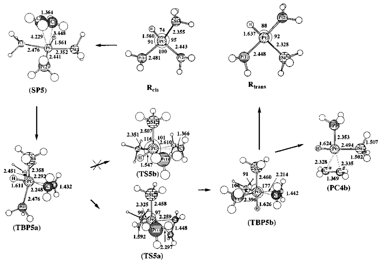
Fig. 2. Geometry changes of \text{C}_2\text{H}_4 -promoted cis - trans isomerization of \text{PtH}(\text{SiH}_3)(\text{PH}_3)_2 (bond length in Å and bond angle in degree).
