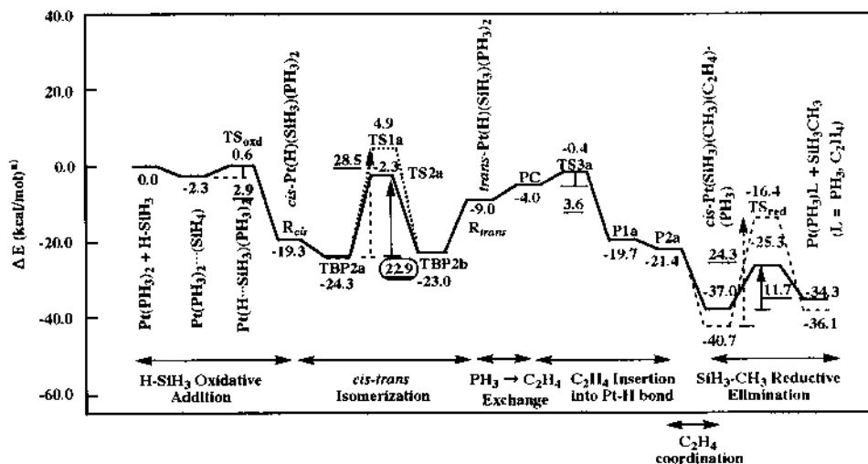
(A) Chalk-Harrod mechanism including the cis-trans isomerization
