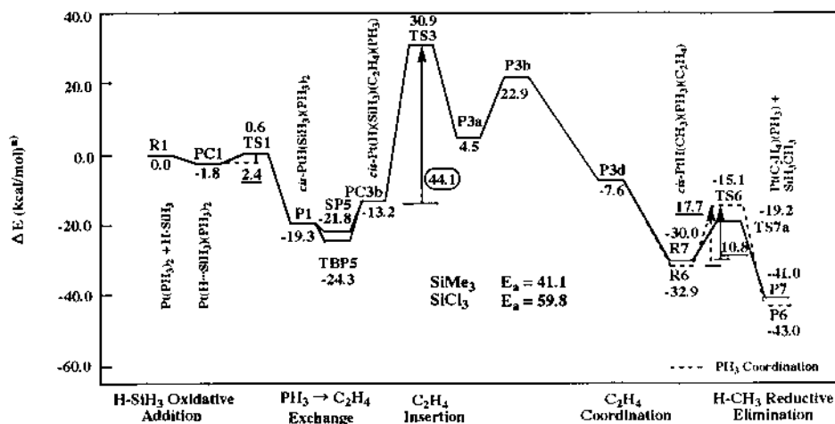
(B) Modified Chalk-Harrod mechanism
