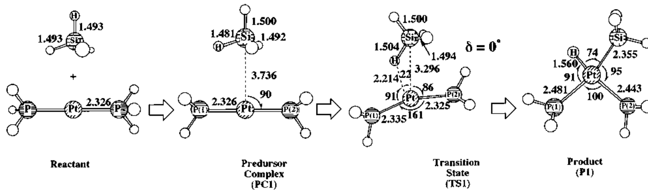
Fig. 1. Geometry changes in the Si-H oxidative addition of \text{SiH}_4 to \text{Pt}(\text{PH}_3)_2 (bond length in Å and bond angle in degree).
