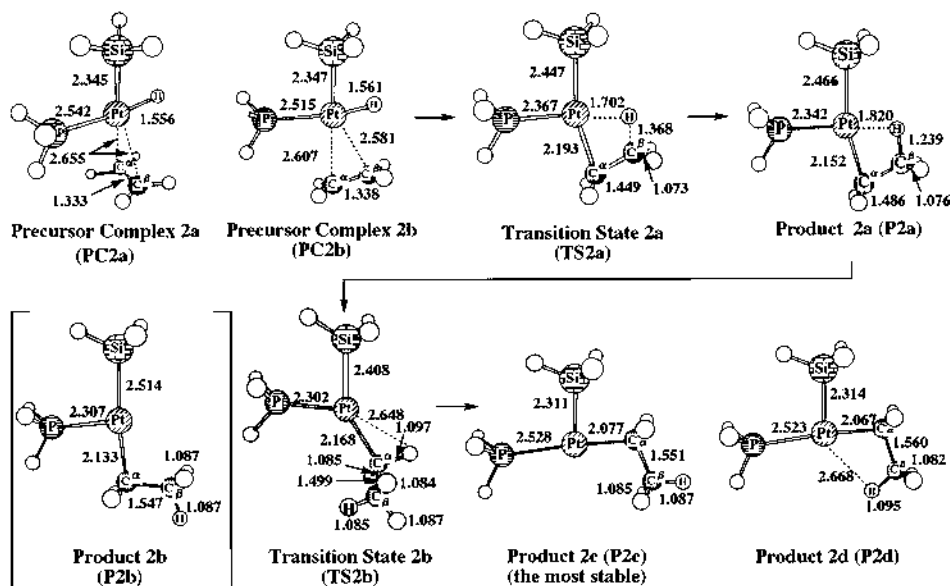
Fig. 3. Geometry changes in the ethylene insertion into the Pt-H bond of cis -PtH(SiH 3 )(PH 3 )(C 2 H 4 ) (bond length in Å and bond angle in degree).
