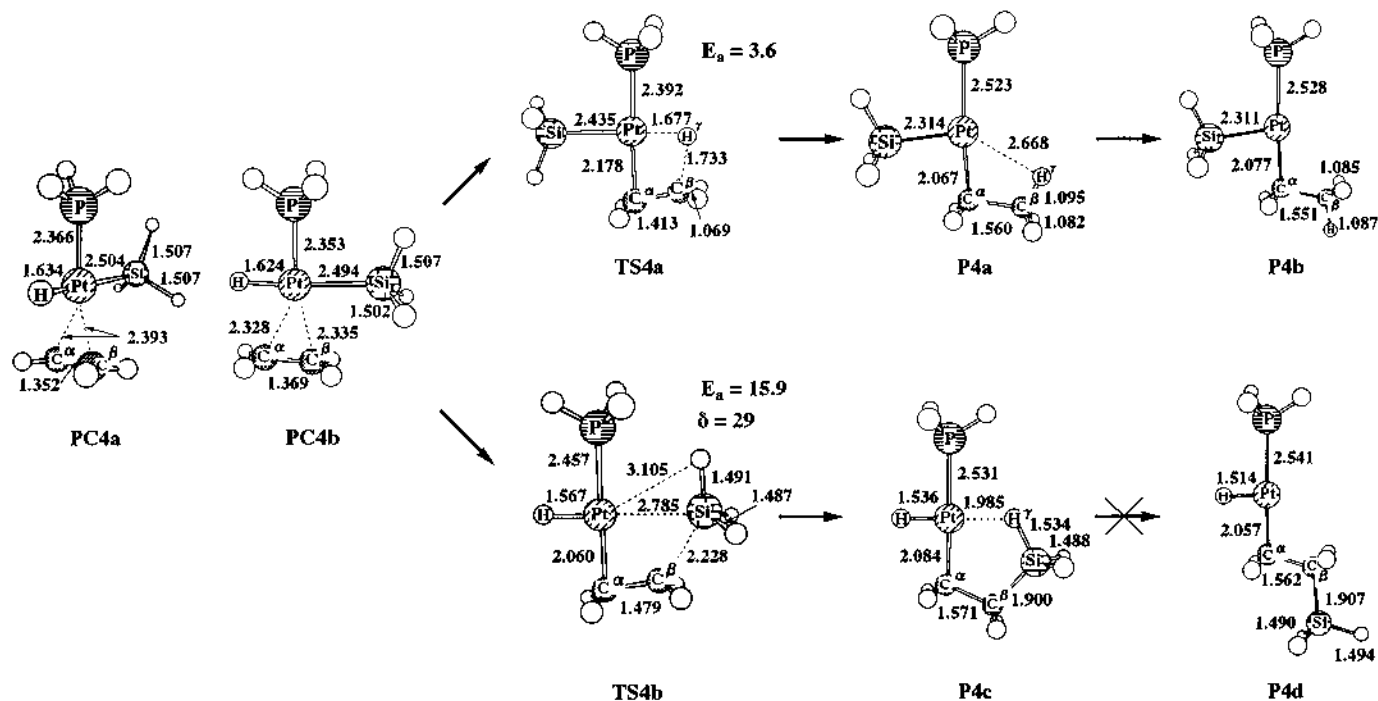
Fig. 5. Geometry changes in the ethylene insertion into Pt-H and Pt-SiH 3 bonds of trans -PtH(SiH 3 )(PH 3 )(C 2 H 4 ) (bond length in Å and bond angle in degree).
