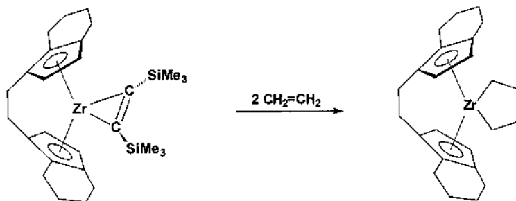
Fig. 19. Synthesis of metallacyclopentane zirconocene procatalyst.
