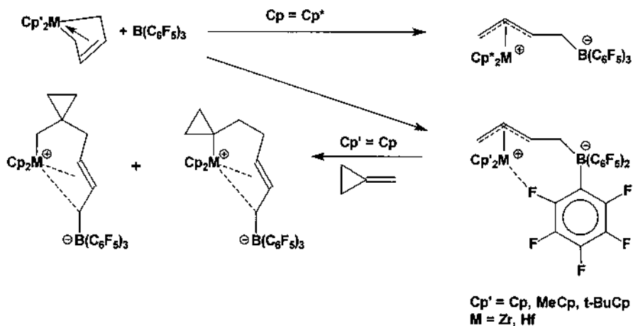
Fig. 34. Reactions of \text{Cp}'_2\text{Zr}(\text{butadiene}) with \text{B}(\text{C}_6\text{F}_5)_3 .
