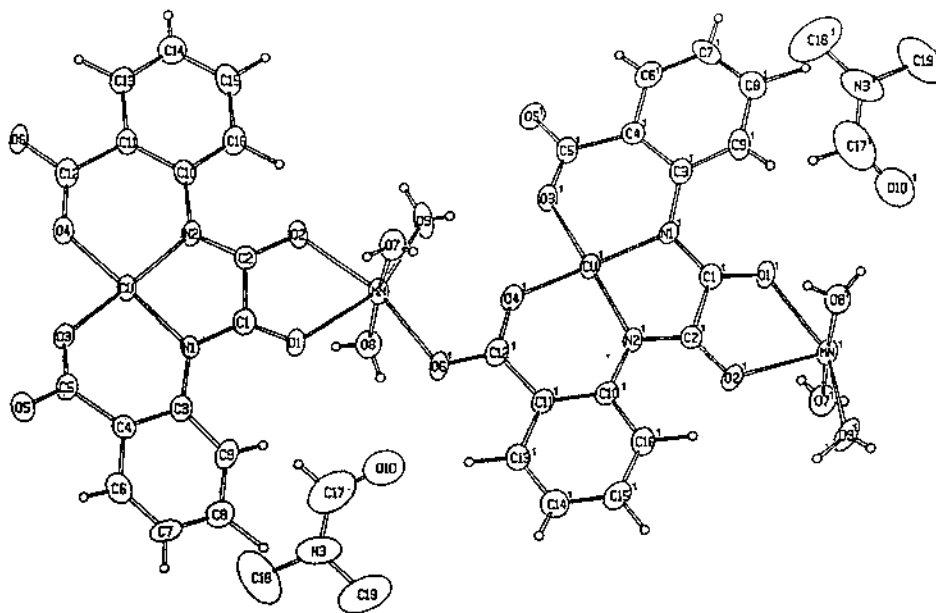
Fig. 25. Perspective drawing of a fragment of the alternating bimetallic chain [\text{MnCu}(\text{obbz})(\text{H}_2\text{O})_3]\cdot\text{dmf} . (Reprinted with permission from Lloret et al. [63]. Copyright © 1993 American Chemical Society.)
