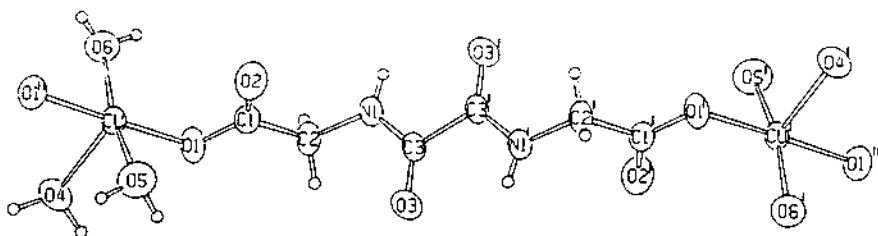
Fig. 22. Perspective drawing of a fragment of the copper(II) chain [\text{Cu}(\text{H}_2\text{glyox})(\text{H}_2\text{O})_3] \cdot 4\text{H}_2\text{O} . (Reprinted with permission from Lloret et al. [20]. Copyright © 1992 American Chemical Society.)
