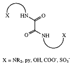
Scheme 2.
