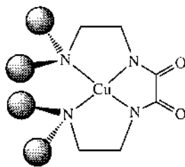
Scheme 12.
