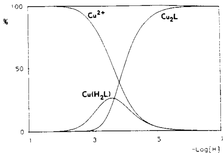
Fig. 20. Distribution diagram for the system \text{Cu}^{2+} –glyox ^{4-} – \text{H}^+ as a function of pH ( c_{\text{Cu}} = c_{\text{L}} = 5 \times 10^{-3} \text{ mol dm}^{-3} ). (Reprinted with permission from Lloret et al. [20]. Copyright © 1992 American Chemical Society.)
