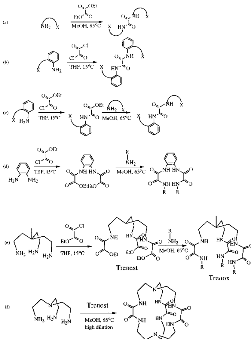
Scheme 3.
