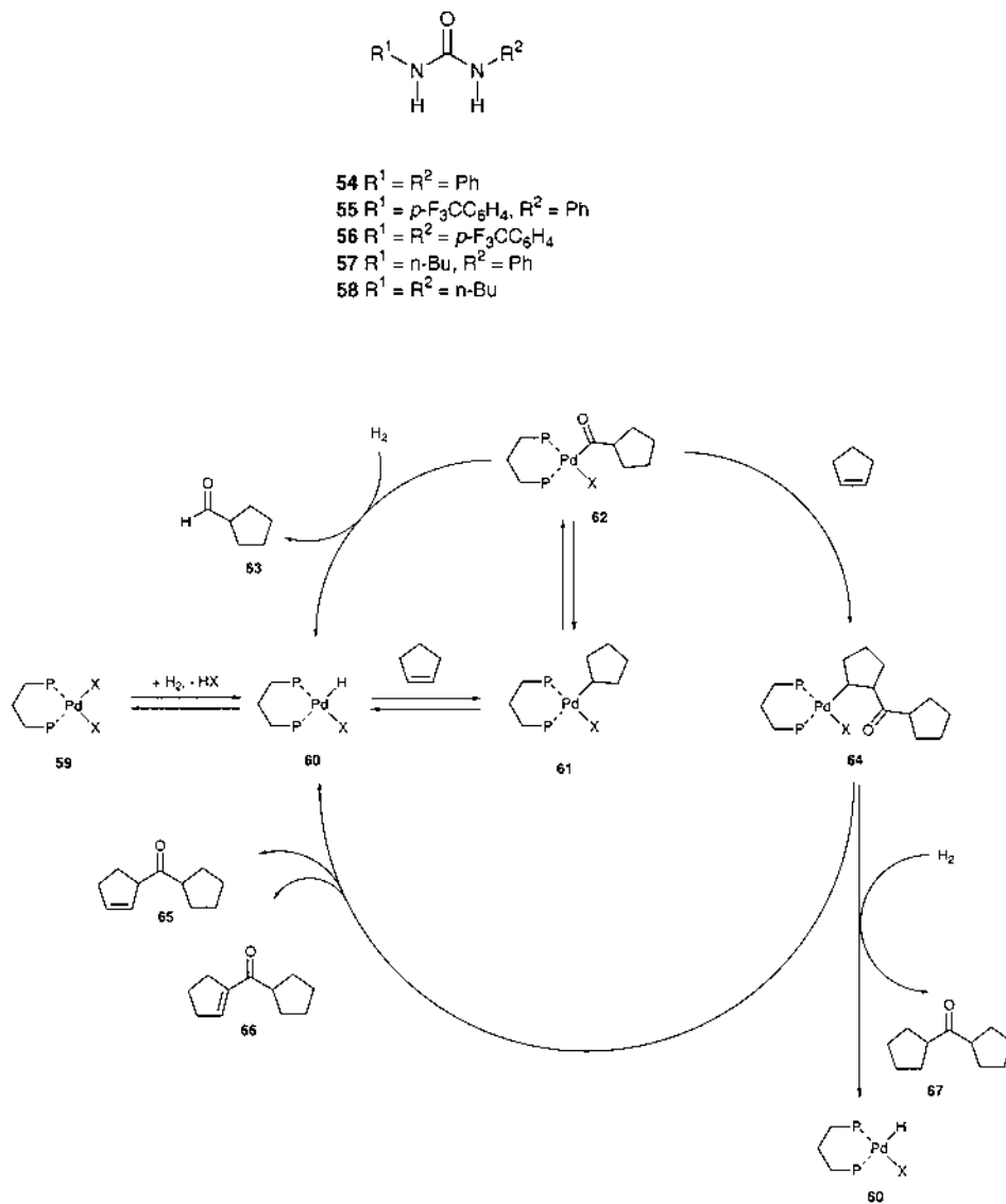
Scheme 7. Catalytic cycle for the \text{Pd}(\text{II}) catalyzed hydrocarbonylation of cyclopentene.
