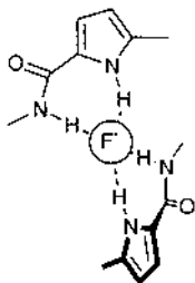
Fig. 6. A tetrahedral arrangement of hydrogen bonds in the catenane 32 leads to remarkably stable anion complexes.
