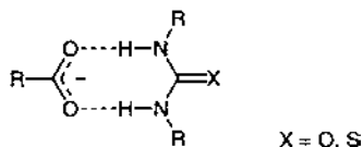
Fig. 7. The ideal two-point interaction between (thio)urea and carboxylate anions.
