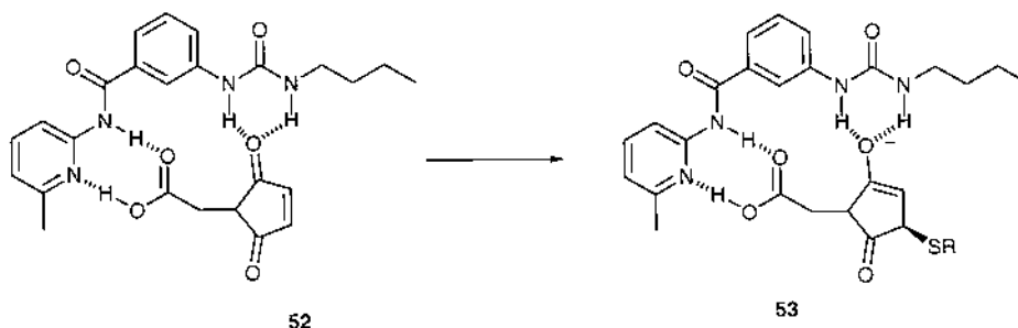
Scheme 6. Acceleration of a 1,4-addition reaction by stabilization of an enol intermediate.
