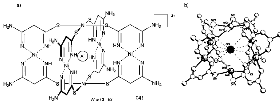
Fig. 22. The structure and crystal structure of the anion directed cage [Ni_6(atu)_8Cl]Cl_3 141 . (Reproduced with permission from Angew. Chem. Int. Ed. Engl. 37 (1998) 1258, Copyright 1998, Wiley-VCH.)
