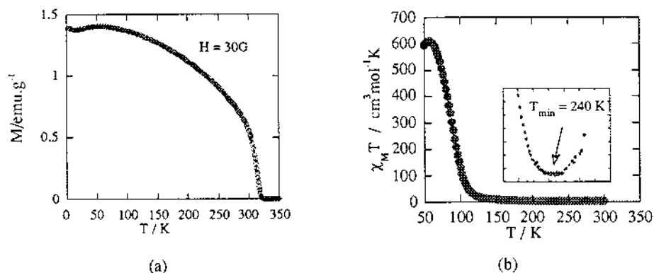
Fig. 7. Thermal variation of (a) the magnetisation in \text{V(II)}_{0.42}\text{V(III)}_{0.58}[\text{Cr(III)(CN)}_6]_{0.86} \cdot 2.8\text{H}_2\text{O} ; (b) the \chi_M T product in \{\text{VO(IV)}\}[\text{Cr(III)(CN)}_6]_{2/3} \cdot 10/3\text{H}_2\text{O} .
