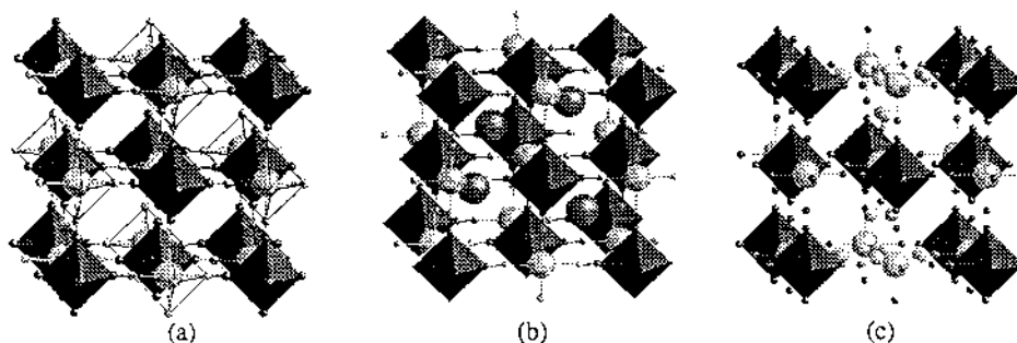
Fig. 1. Typical structures of cubic Prussian blue: (a) A(III)[B(III)(CN)_6] , A_1B_1 ; (b) Cs(I)A(II)[B(III)(CN)_6] , Cs_1A_1B_1 ; (c) \{A(II)_3\}[B(III)(CN)_6]_2 \cdot xH_2O , A_3B_2 . [B(CN)_6] are the dark solid octahedra surrounded by CN (very small spheres), A are the light small spheres, C are the grey medium size spheres in (b); in (c) H_2O are shown by the small light-grey spheres.
