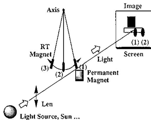
Fig. 11. Scheme of a device using the properties of a r.t. magnet to transform light in mechanical energy.
