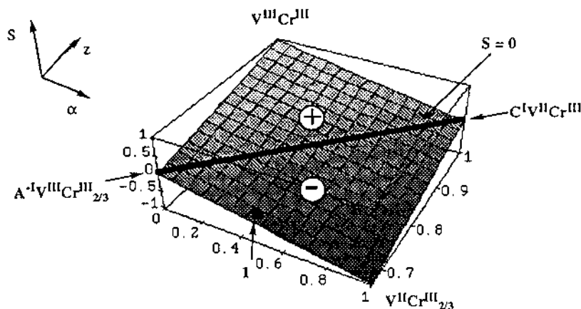
Fig. 8. Variation of the spin values S versus z and \alpha parameters for compounds C(I)_y V(II)_x V(III)_{1-x} \alpha [Cr(III)(CN)_6]_z \cdot nH_2O . 1 is in the part of the plane where the total spin has the same direction as the vanadium spins.
