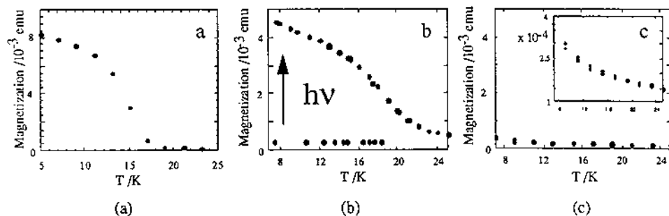
Fig. 12. Magnetisation and photo-induced magnetisation of: (a) compound 6; (b) compound 8; and (c) compound 7 (insert: y is scaled \times 10 ).
