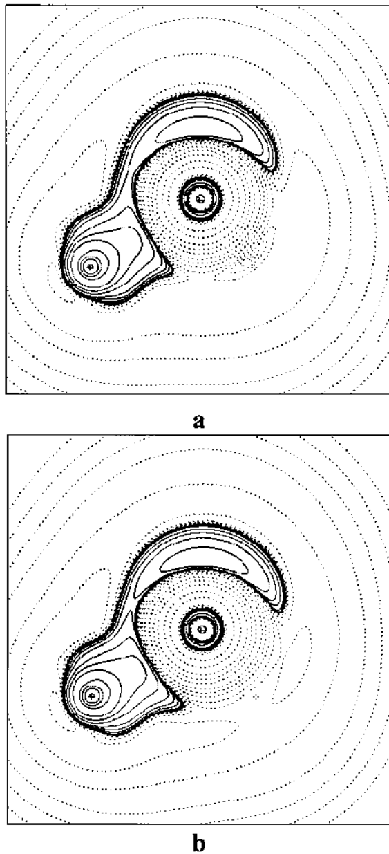
Fig. 3. Maps of the Laplacian of the electron density and (a) of the conditional pair density for electrons of both spins, (b) for a plane of the \text{PH}_3 molecule containing a single proton, a \sigma_v symmetry plane. The solid contours are for regions where each function is concentrated, i.e. L(\mathbf{r}) > 0 in the case of the density, the dashed contours for regions where the functions are depleted. The reference electron for the conditional density display is placed at the position of an out-of-plane proton, where L(\mathbf{r}) exhibits a very pronounced local maximum, as demonstrated in (a). Thus, when the Fermi density of the reference electron is very localized, as it is in this case, then the conditional density approaches the electron density outside of the region of localization and the Laplacians of the two functions not only display the same local maxima at the same locations, but approach one another in value.
