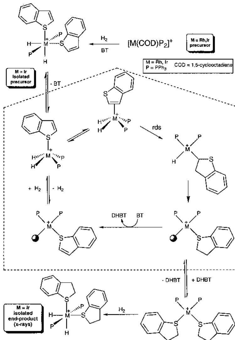
Scheme 17. The mechanism for the hydrogenation of benzothiophene (BT) catalyzed by [\text{Rh}(\text{H})_2(\text{BT})_2(\text{PPh}_3)_2]^+
