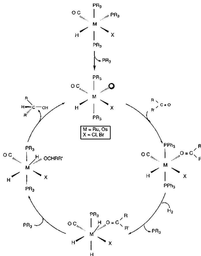
Scheme 10. The mechanism for the hydrogenation of aldehydes catalyzed by MHX(CO)(PPh_3)_3 ( M = Ru, Os ; X = Cl, Br ).
