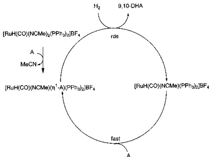
Scheme 15. The mechanism for the hydrogenation of acridine (A) catalyzed by [\text{RuH}(\text{CO})(\text{MeCN})_2(\text{PPh}_3)_2]^+ .
