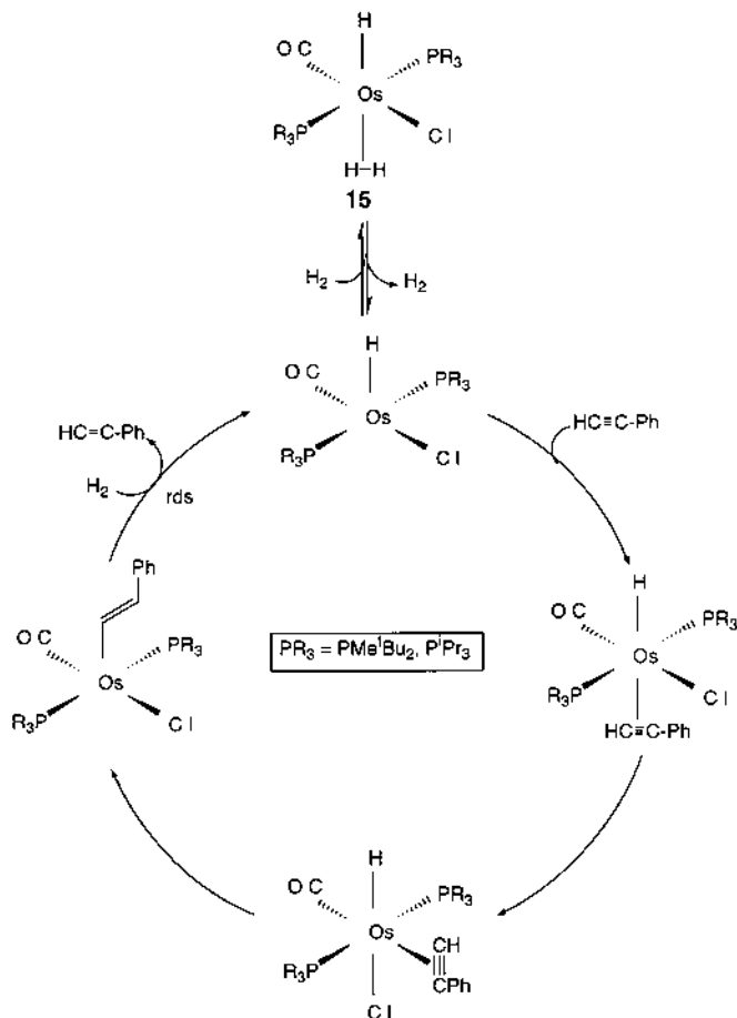
Scheme 8. The mechanism for the hydrogenation of phenylacetylene catalyzed by \text{OsHCl}(\text{CO})(\text{PR}_3)_2 ( \text{R} = \text{P}^{\text{Me}}\text{Bu}_2, \text{P}'\text{Pr}_3 ).
