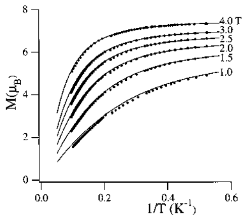
Fig. 20. Magnetization curve vs. the inverse of the temperature for the Ni(II) complex of the series [M_4(H_2O)_2(PW_9O_{34})_2]^{10-} at different magnetic fields. The solid line represents the calculated behavior with the magnetic parameters given in the text.
