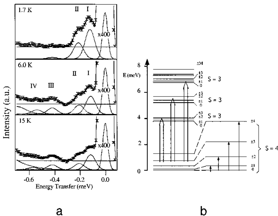
Fig. 21. (a) Inelastic neutron scattering spectra of the deuterated sample K_6Na_4[Ni_4(H_2O)_2(PW_9O_{34})_2 \cdot 24H_2O] measured on IN5 at ILL, Grenoble, France, with an incident neutron wavelength of 6.5 Å at temperatures of 1.7, 6.0 and 15 K; (b) energy spectrum of the Ni_4O_{16} ferromagnetic cluster indicating the allowed magnetic excitations.
