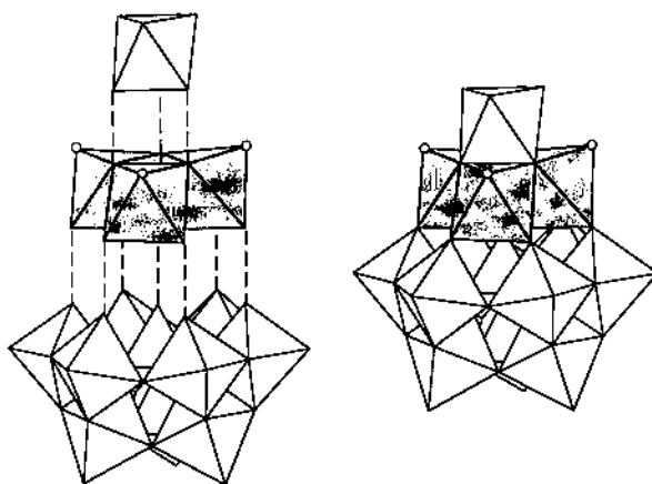
Fig. 8. Structure of the [\text{Ni}_3(\text{H}_2\text{O})_3(\text{PW}_{10}\text{O}_{39})\text{H}_2\text{O}]^{7-} complex.
