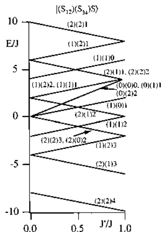
Fig. 19. Energies of the spin states of a rhomb-like cluster of ferromagnetically coupled S=1 spins as a function of the J'/J ratio. The wave functions are labeled according to the Kambe-type coupling scheme ( S_{12} and S_{34} are intermediate spin values and S is the total spin).
