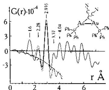
Fig. 3. G(r) for bis-(triphenylphosphinegold)malonitrile. Here and in analogous figures: solid line is an experimental difference RDF; dashed-and-dotted line is a model contribution of distances between the heavy metal atoms (here Au–Au); short dashes show a sum of all contributions of near interatomic distances taken into account in a model RDF calculation (here AuAu + AuP + AuC); long dashes show a zero line for absolute intensities of peaks in G(r) (see Section 2, the last paragraph). When the dashed-and-dotted and dashed lines coincide in any r -region in the RDF of a model, the common line in such a region is shown in the figures with the one of these types of dashes. A structure model is shown near the RDF which corresponds to the RDF simulation. Arrows indicate positions of maxima of peaks of an experimental G(r) . All G(r) are given in \text{e}^2 \text{Å}^{-1} .
