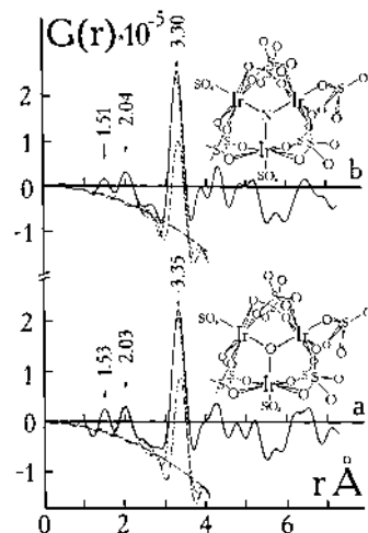
Fig. 9. G(r) of K_6H_4[Ir_3(III,III,IV)O(SO_4)_9] \cdot 3H_2O (a) and of (NH_4)_{10}[Ir_3(III,IV,IV)N(SO_4)_9] (b). The oxygen atoms of sulfate groups, that are located closer to the reader, are designated with the larger symbols than those located more far.
