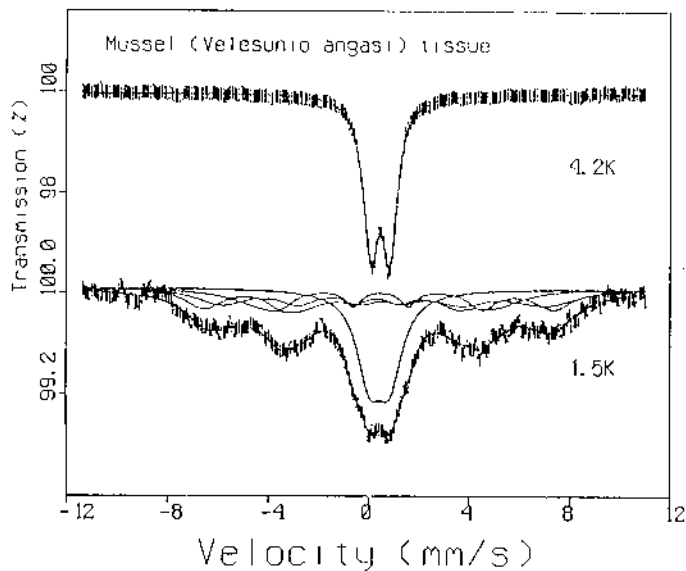
Fig. 9. Mössbauer spectra of tissue granules of freshwater mussel Velutunio angasi at 4.2 and 1.5 K.
