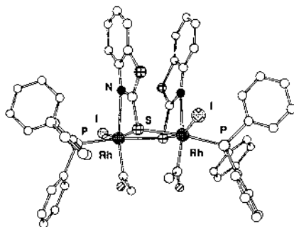
Fig. 29. Molecular structure of [\text{Rh}_2(\mu\text{-bztat})_2(\text{COMe})_2(\text{I})_2(\text{PPh}_3)_2] .
