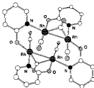
Fig. 19. Molecular structure of [\text{Rh}_4(\mu\text{-OPy})_4(\mu\text{-CO})_2(\text{CO})_4] .
