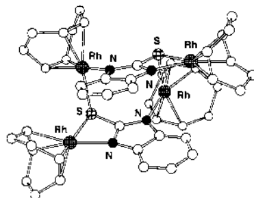
Fig. 23. Molecular structure of [\text{Rh}_4(\mu\text{-bzint})_2(\text{COD})_4] .
