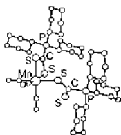
Fig. 4. Molecular structure of cation [Mn(CO)_3(\eta^2-S_2CPCy_3)(\eta^1-S_2CPCy_3)]^+ .
