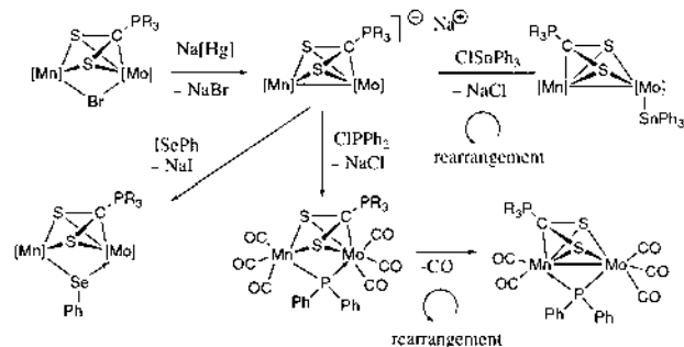
Scheme 33.
