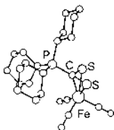
Fig. 5. Molecular structure of Fe(CO) 3 ( \eta^3 -S 2 CPCy 3 ).
