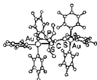
Fig. 6. Molecular structure of [\text{Au}(\text{C}_6\text{F}_5)_3]_2(\mu\text{-S}_2\text{CPEt}_3) .
