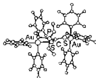
Fig. 3. Molecular structure of Pt(C_6F_5)_2(CO)(\eta^1-S_2CPCy_3) .
