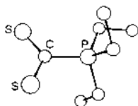
Fig. 1. Molecular structure of S_2CPEt_3 .
