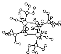
Fig. 7. Molecular structure of [\text{Mo}(\text{CO})_2(\text{PEt}_3)(\mu\text{-S}_2\text{CPEt}_3)]_2 .
