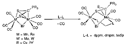
Scheme 15.
