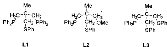
Fig. 11. The ligands L1, L2 and L3.
