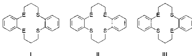
Fig. 15. Three types of 14-membered macrocyclic phosphino–thioethers and arsino–thioethers.
