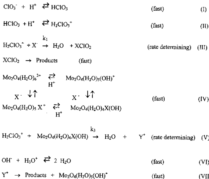
Scheme 3.
