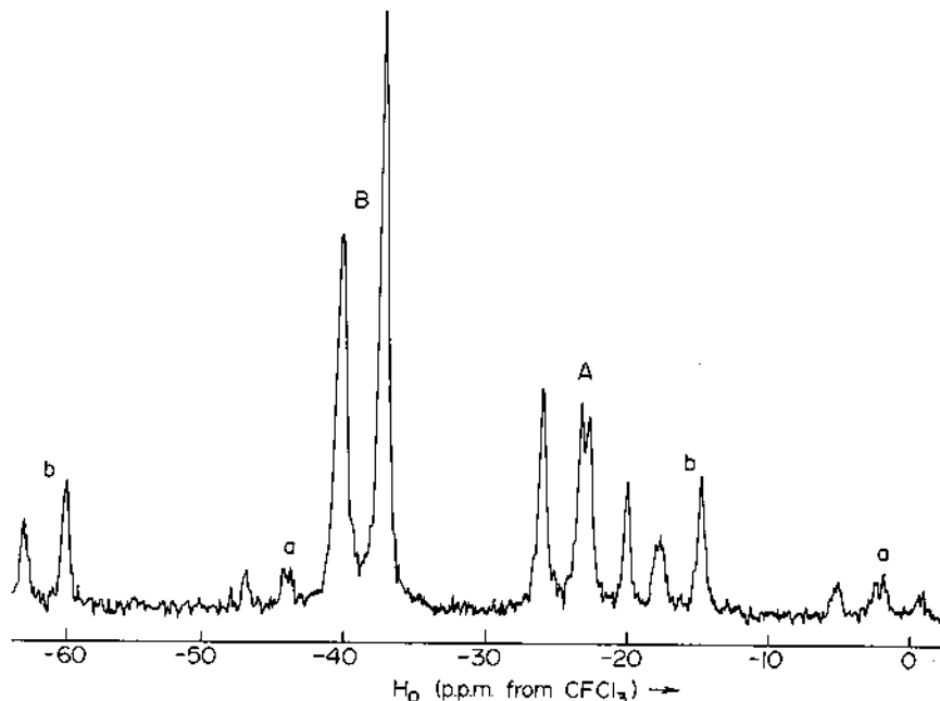
Fig. 2. ^{19}\text{F} -NMR spectrum (56.4 MHz, 26^\circ\text{C} ) of the \text{XeF}_3^+ cation (0.20 M \text{XeF}_4 and 0.50 M \text{XeF}_2 in \text{SbF}_5 solution): (A) axial fluorines and (a) ^{129}\text{Xe} satellites; (B) equatorial fluorine and (b) ^{129}\text{Xe} satellites [33]. The chemical shift scale must be multiplied by -1 to conform with the present IUPAC convention.
