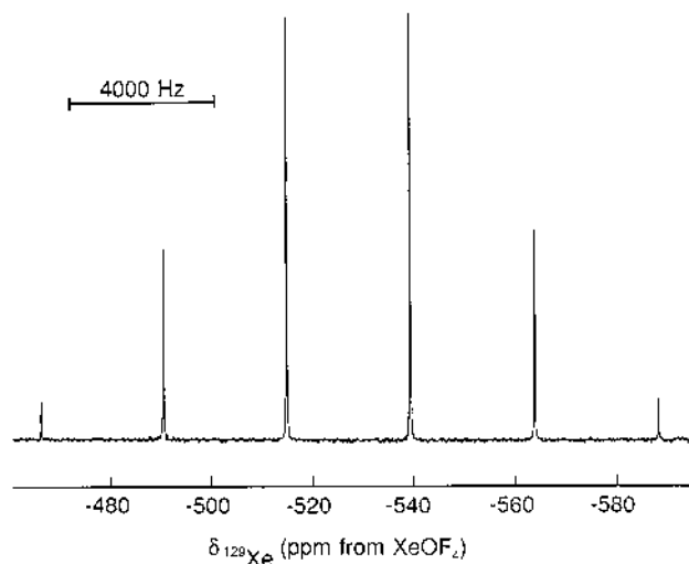
Fig. 14. ^{129}\text{Xe} -NMR spectrum (139.05 MHz, 24°C) of a saturated solution of \text{N}(\text{CH}_3)_4^+\text{XeF}_5^- in \text{CH}_3\text{CN} containing an equimolar amount of \text{N}(\text{CH}_3)_4^+\text{F}^- [95].
