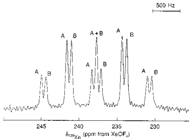
Fig. 4. ^{129}\text{Xe} -NMR spectrum (139.051 MHz, 30°C) of ^{17}\text{O} - (26.5%) and ^{18}\text{O} -enriched (37.0%) \text{XeOF}_3^+ and \text{SbF}_6^- (0.33 M) and \text{XeF}_2 (1.7 M) dissolved in \text{SbF}_5 solvent; resolution enhanced spectrum obtained by Fourier transformation of the free induction decay using a Gaussian fit: (A) \text{Xe}^{16}\text{OF}_3^+ , (B) \text{Xe}^{18}\text{OF}_3^+ [38].
