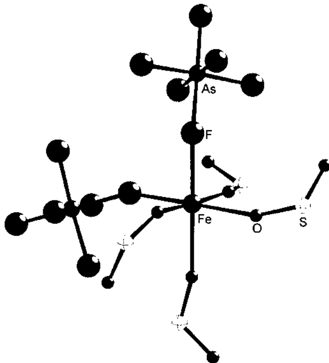
Fig. 12. Crystal structure of [\text{Fe}(\text{OSO})_4(\text{FAsF}_5)_2] [78].
