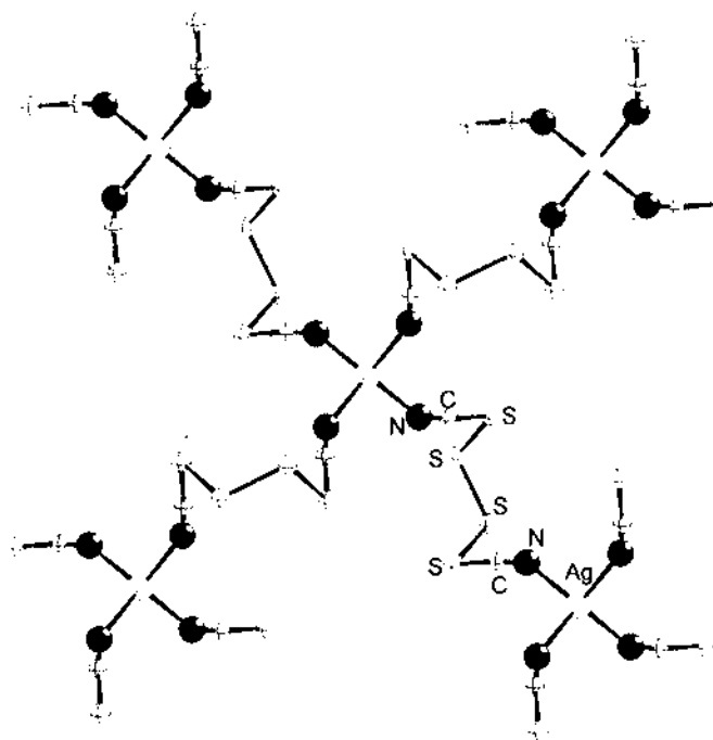
Fig. 19. Crystal structure of [\text{Ag}(\text{NCS}_4\text{CN})_{4/2}]_n(\text{AsF}_6)_n [97].
