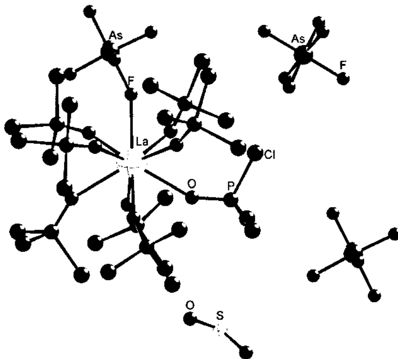
Fig. 32. Crystal structure of [\text{La}(\text{OPCl}_3)_8(\text{FAsF}_5)](\text{AsF}_6)_2 [77].
