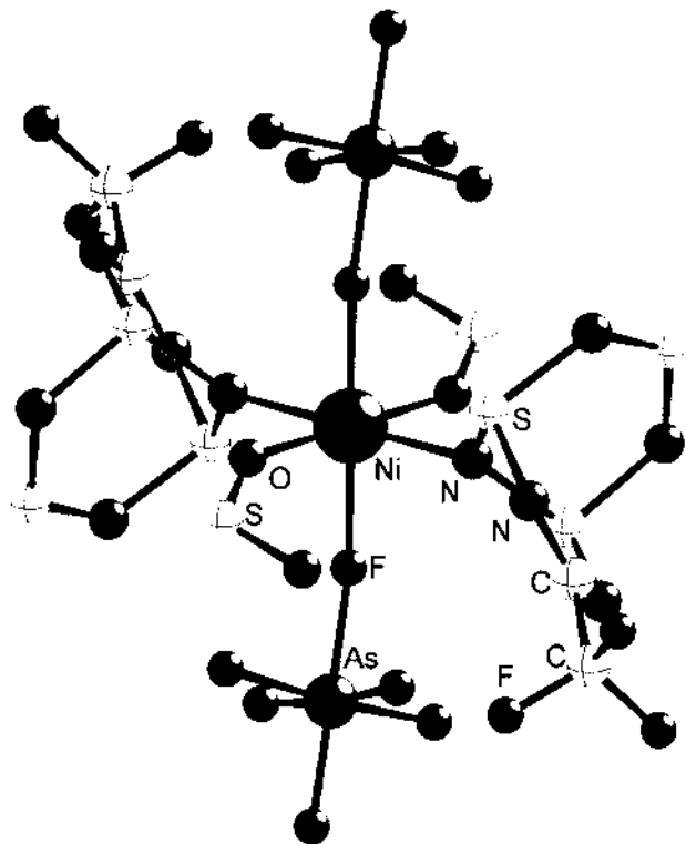
Fig. 33. Crystal structure of [\text{Ni}(\text{CF}_3\text{CN}_4\text{S}_3)_2(\text{OSO})_2(\text{FAsF}_5)_2] [133].
