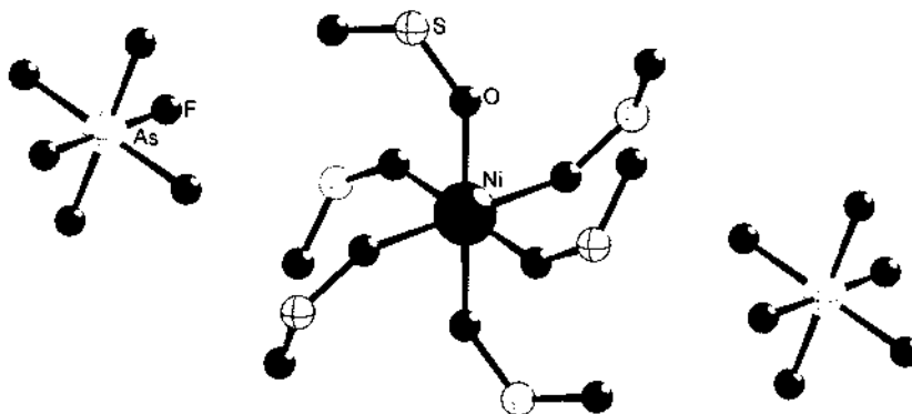
Fig. 10. Crystal structure of [\text{Ni}(\text{OSO})_6](\text{FAsF}_3)_2 [78].
