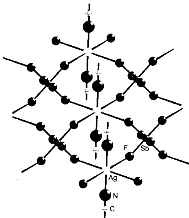
Fig. 16. Crystal structure of \{[\text{Ag}(\text{NCH})_2](\text{SbF}_6)_{4/4}\}_n [92].
