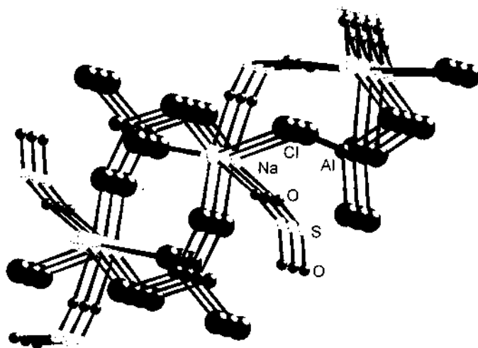
Fig. 3. Crystal structure of [Na(SO 2 ) 1.5 AlCl 4 ] n [40].
