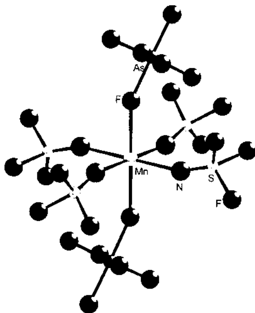
Fig. 27. Crystal structure of [\text{Mn}(\text{NSF}_3)_4(\text{FAsF}_5)_2] [127].
