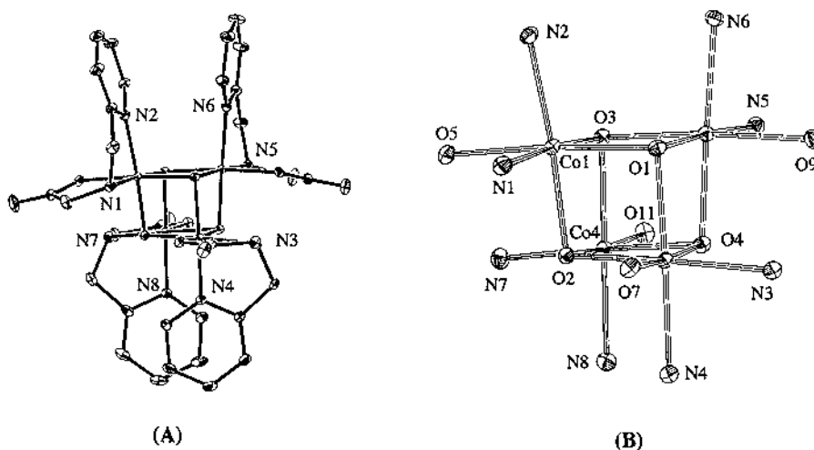
Fig. 7. Perspective view of the isolated [\text{Co}_4(\text{pg})_4(\mu_3\text{-O})_4] isomer. (A) The structure of the tetranuclear complex and (B) the complete cubane core of the complex.
