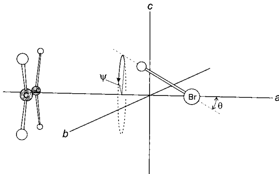
Fig. 2. The model of C_2H_4 \cdots HBr used to determine the geometry of the complex from its zero-point moments of inertia. The angular oscillation of the HBr subunit illustrated is two-dimensionally isotropic in the bc plane and is defined in terms of the angles \psi and \theta . This diagram is drawn to scale, except for the angle \theta , which is exaggerated with respect to \theta_{av} = \cos^{-1} \langle \cos^2 \theta \rangle^{1/2} , determined from \chi_{aa} , for clarity.
