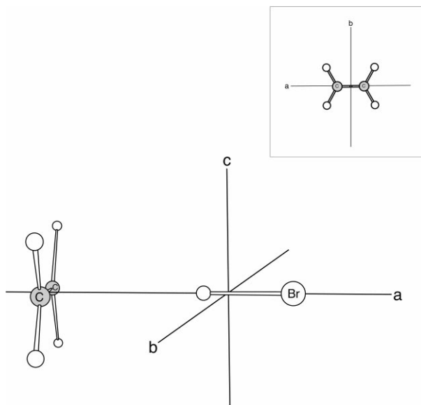
Fig. 1. The equilibrium angular geometry of the complex C 2 H 4 ...HBr. The diagram is drawn to scale and the positions of the principal inertia axes a , b and c are indicated. The insert shows the directions of the principal inertial axes a and b in the free ethene molecule.
