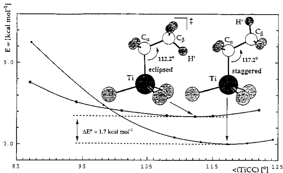
Fig. 9. Variation of the total energy with \text{Ti-C-C} angle in \text{EtTiCl}_3 for eclipsed and staggered conformers. Primes indicate the location of an atom either in (') or out of (") the \text{C}_s symmetry plane of the molecule. Reproduced with permission from Ref. [61].
