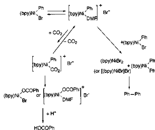
Scheme 13.
