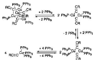
Scheme 6.
