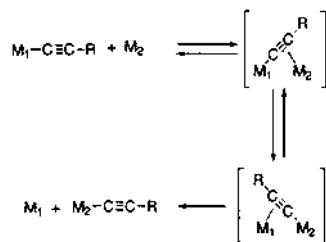
Scheme 9.
