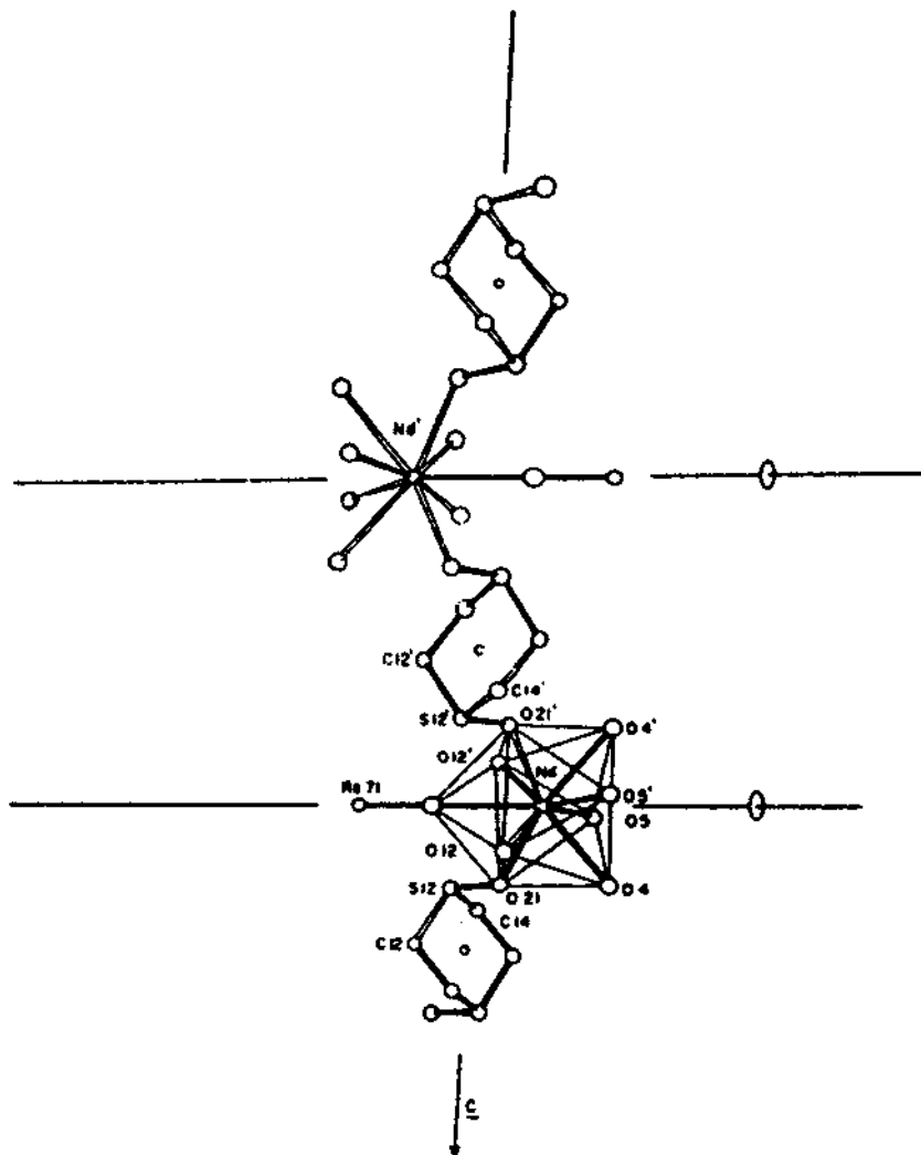
Fig. 7. Projection of the polyhedron chain of the complex of neodymium perhenate with TDTD (primed names refer to symmetrically related atoms) (Ref. [38] p. 212).
