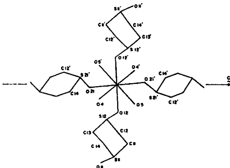
Fig. 8. Projection down b -axis showing the TDMD groups and the oxygen water molecules coordinated to the \text{Nd}^{3+} ions in the polyhedra of Fig. 7 (Ref. [38] p. 213).
