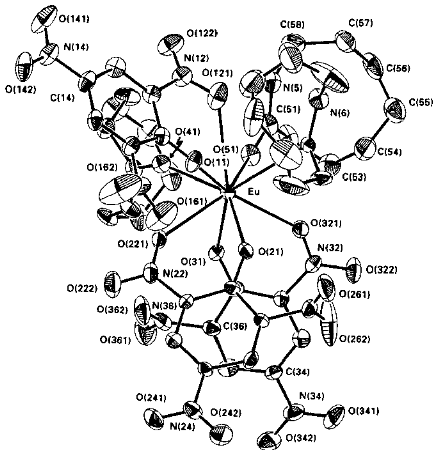
Fig. 12. Structure of the complex of formula [Eu(pic)_3(AZA)_3] (Ref. [46] p. 3521).
