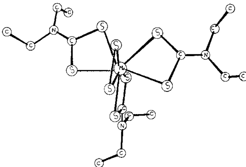
Fig. 5. The monomer [Mo(S_2)(dtc)_3] [51,52].
