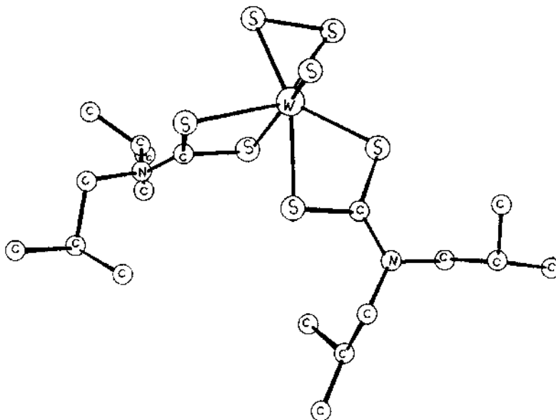
Fig. 6. Heptacoordinate tungsten in [WS(S_2)(dte)_2] [51,52].
