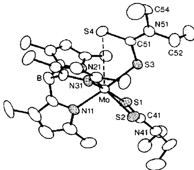
Fig. 4. A view of the structure of [\{HB(Me_2pz)_3\}Mo(\mu_2-Me_2dtc)(\mu_1-Me_2dtc)] [49,50].
