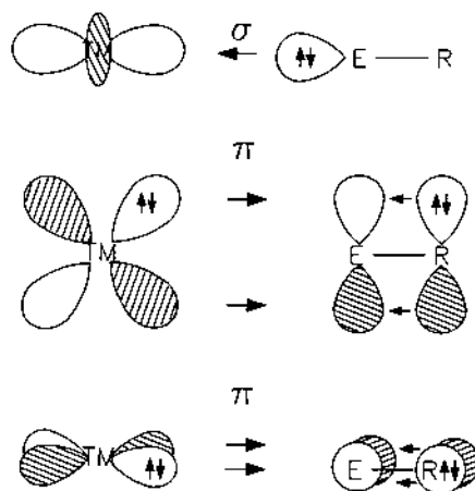
Fig. 1. Principle donor–acceptor interactions in transition metal Group 13 diyl complexes L_n\text{TM-ER} where \text{R} carries the \pi lone-pair electrons.
