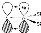
Fig. 8. Schematic representation of the dominant intraligand N → E \pi -donation in EN(SiH 3 ) 2 .
