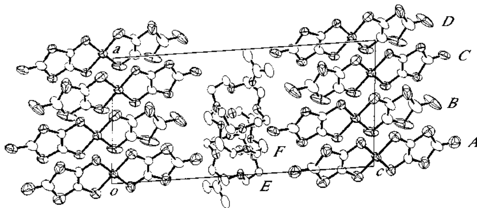
Fig. 1. Unit cell of (Li + ) 2 (12-crown-4) 3 [Ni(dmit) 2 ] 7 (acetone) 2 viewed along the b -axis. The crystallographically identical [Ni(dmit) 2 ] molecules are labeled as A–D and those of 12-crown-4, E–F.
