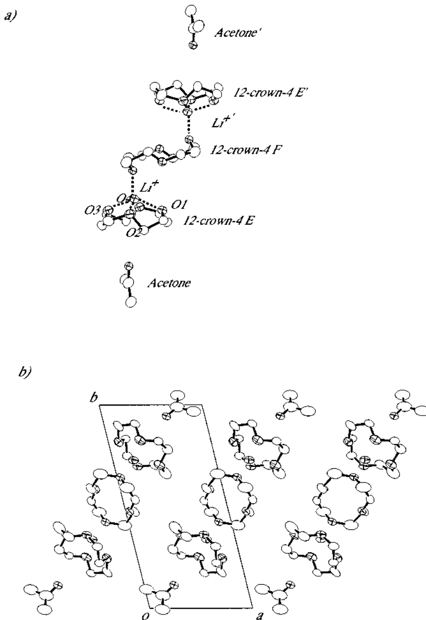
Fig. 2. (a) Dimeric penta-coordinated \text{Li}^+ ion in the SC unit. (b) The SC unit within the a-b plane viewed along the c -axis.
