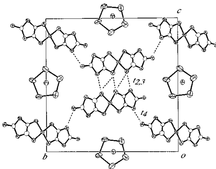
Fig. 4. The crystal structure of \text{Li}_{0.6}(15\text{-crown-5})\text{H}_2\text{O}[\text{Ni}(\text{dmit})_2]_2 viewed along the a -axis.
