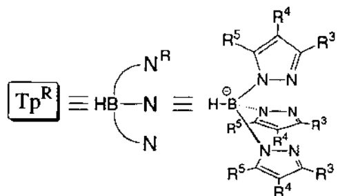
\text{Tp}^{\text{R}} ligands used for Co-dioxygen complexes
