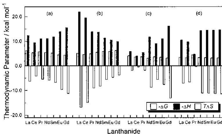
Fig. 8. Thermodynamic parameters for the complexation of light lanthanides with (a) BzA15C5; (b) BzA18C6; (c) BzA21C7; and (d) BzA16C5 in acetonitrile at 25.0^\circ\text{C} .
