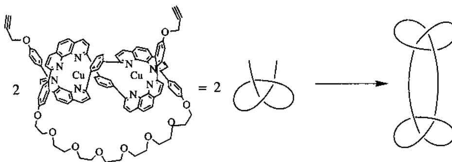
Fig. 10. The first composite knot utilized two two-anchor helical templates.
