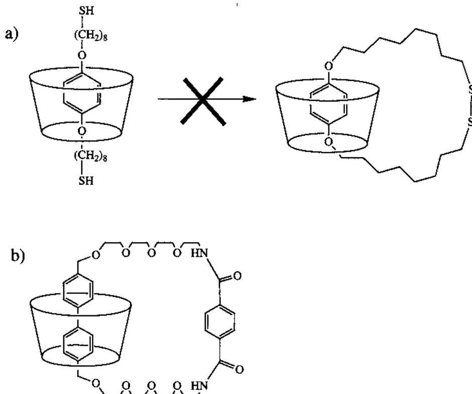
Fig. 24. (a) Luttringhaus' failed cyclodextrin catenane reaction and (b) Stoddart's first successful cyclodextrin [2]-catenane.
