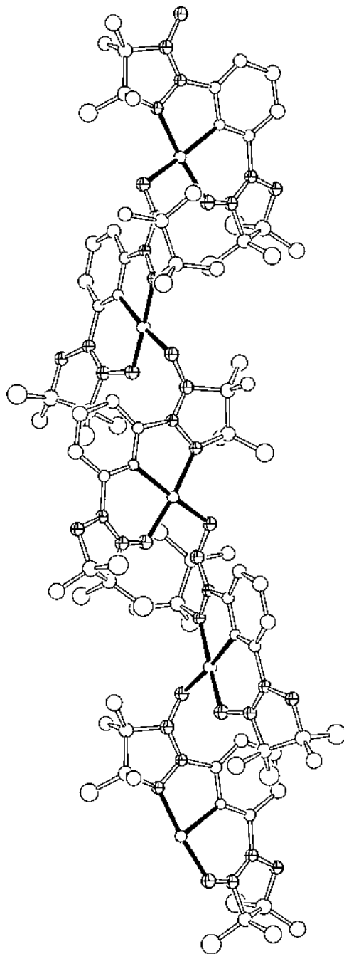
Fig. 9. The radical helix of [Cu(II)(imapy)] + (PF 6 ) - .
