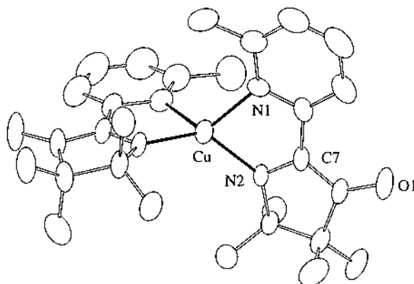
Fig. 1. The structure of [\text{Cu(I)}(\text{immepy})_2]^+ .
