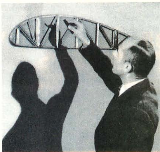
THE EVIDENCE, MR. SHAPIRO Dr. Ascher H. Shapiro, professor of engineering at MIT in 1960, illustrates how the shape of an airfoil generates lift. Air flows over the top of the airfoil faster than the bottom, reducing the air pressure above the airfoil and thus generating lift.
