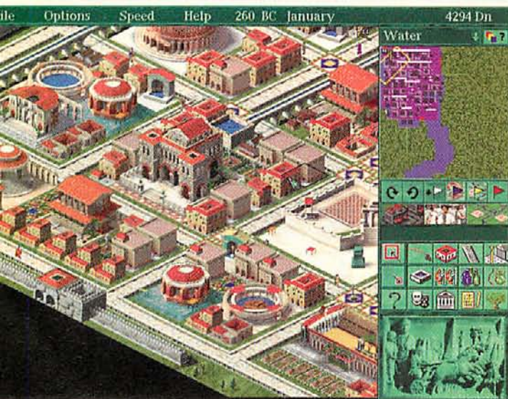
Caesar II 304
