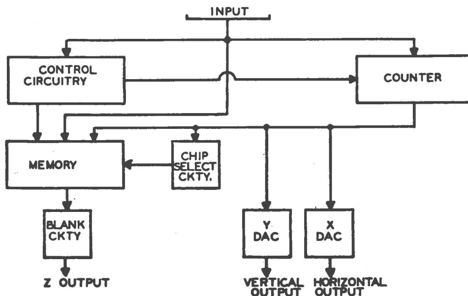
FIGURE 1. DGDOI BLOCK DIAGRAM
