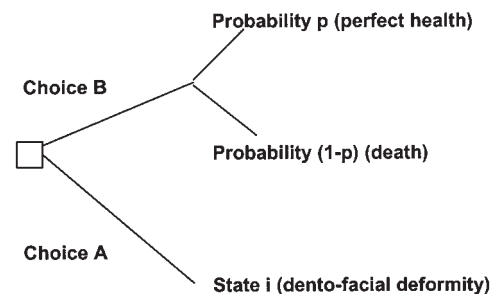
Figure 1 The standard gamble technique.
