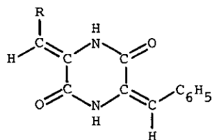
[(3Z, 6E)- 2 ; R=(p)-CH 3 O-C 6 H 4 ]
