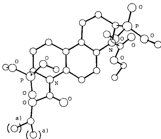
Fig. 1. The molecular structure of 3a
