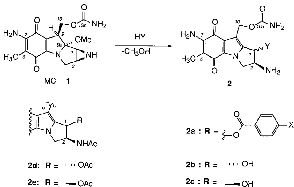
Scheme 1. Formation of Mitosenes
