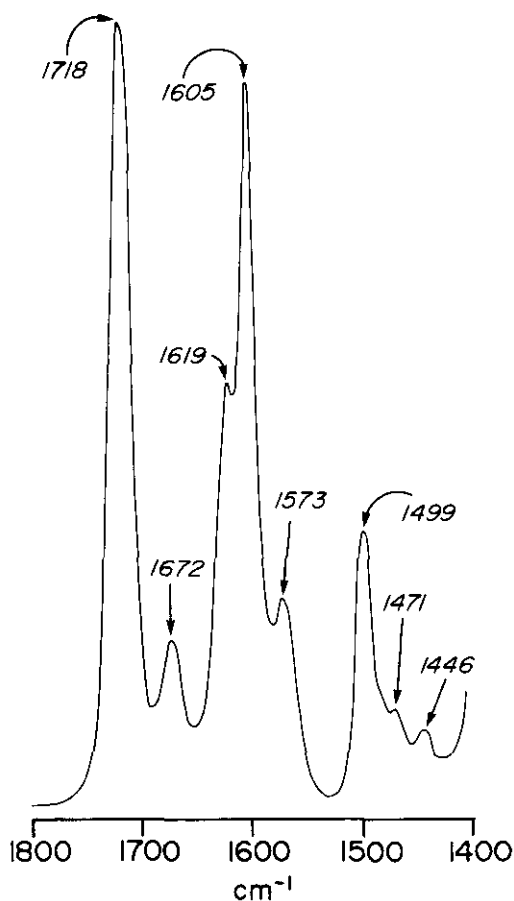
Figure 1. FTIR spectrum of TFA Mitosene 3 , 1800-1400 \text{cm}^{-1} region, (\text{CD}_3)_2\text{SO} solution, internal reflectance microcell.
