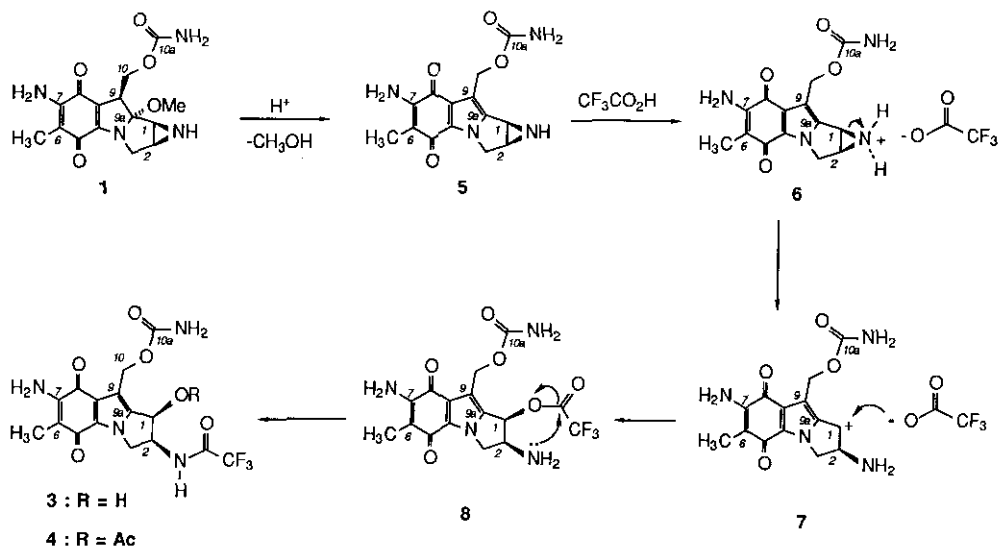
Scheme II. Formation of TFA mitosene 3
