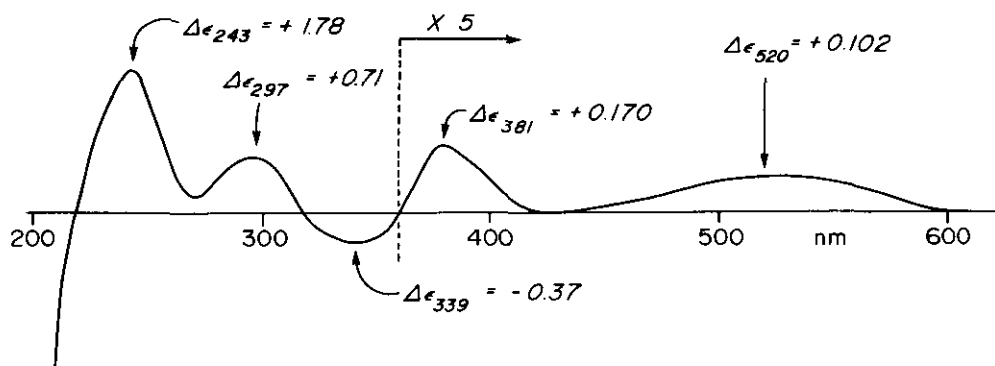
Figure 2. CD spectrum of TFA Mitosene 3 in MeCN.
