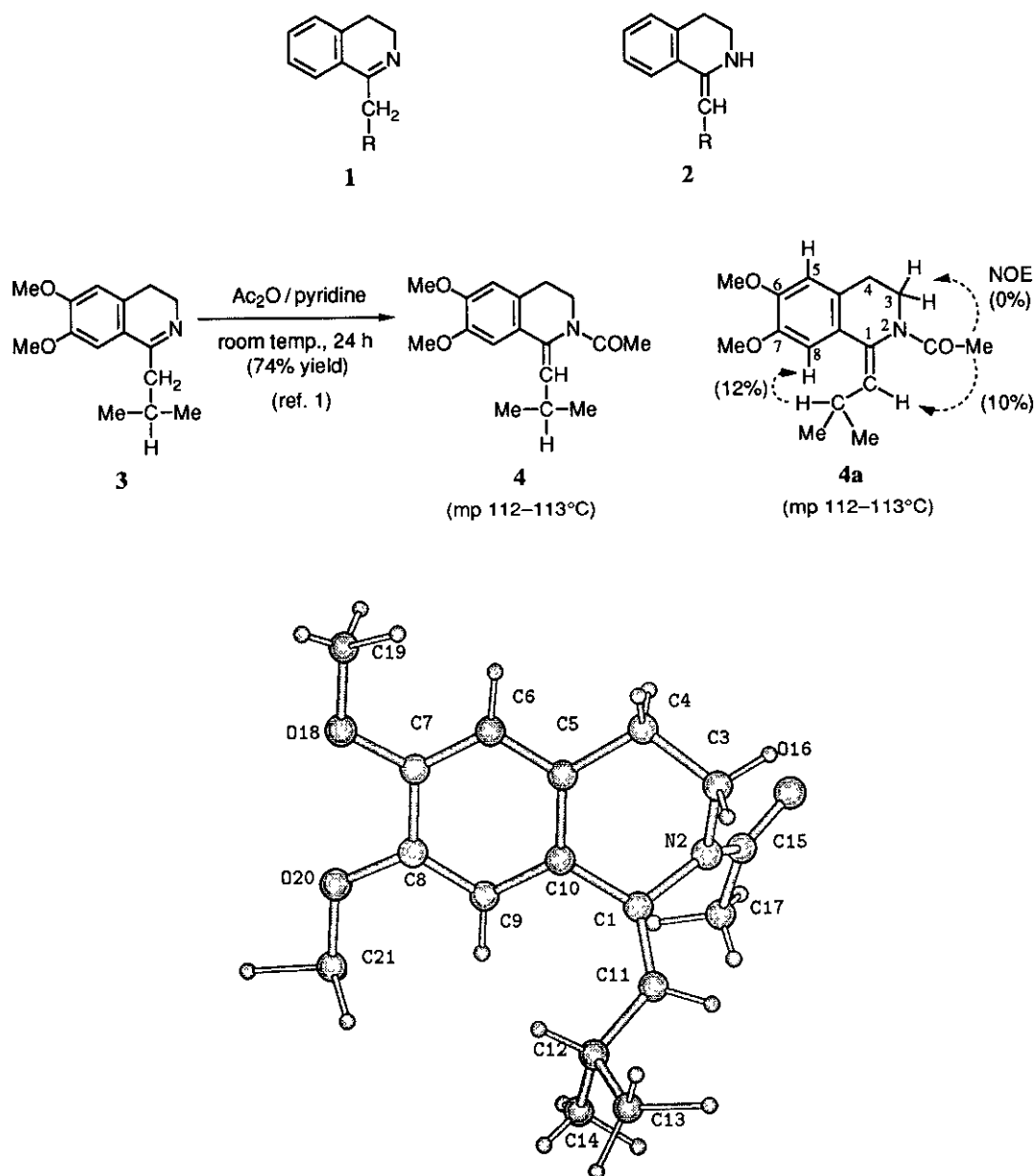
Figure 1. A Parallel View of the Molecular Structure of 4a and the Numbering Scheme Employed for X-ray Crystallographic Data
