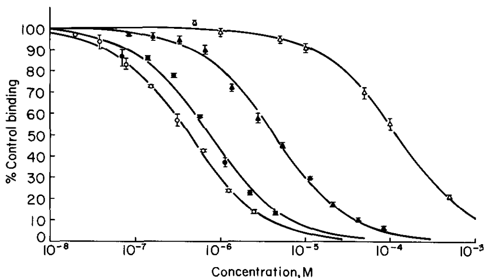
Figure 6. Inhibition of \text{Na}^+, \text{K}^+ -ATPase binding of 25 nM [^3\text{H}] ouabain by marinoobufagin (O), marinoobufotoxin (●), marinoobufagin-3-sulfate (1a) (▲) and, 12 \beta -hydroxy-tetrahydroresibufogenin-3-sulfate (2) (Δ). Binding of [^3\text{H}] ouabain was measured as described in Materials and Methods. Values are averages \pm SD (or range) for 2-3 duplicate measurements at each concentration.
