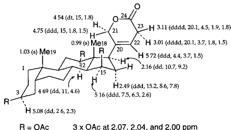
Figure 4. ^1\text{H} -Nmr assignment for 3,12,15-triacetoxytetrahydroresibufogenin (4).
