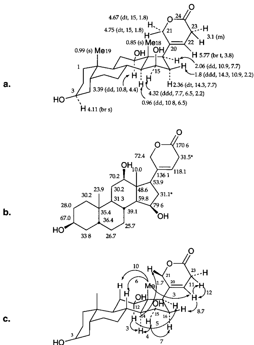
Figure 3. a. ^1\text{H} -Nmr assignment b. ^{13}\text{C} -Nmr assignment c. NOE difference studies of 12 \beta -hydroxytetrahydroresibufogenin ( 3 ).
