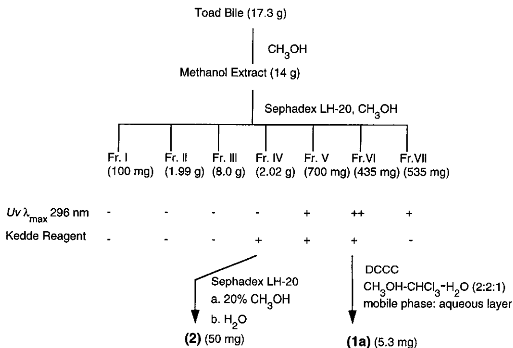
Figure 1. Fractionation and separation of cardiotoxic agents from toad bile.
