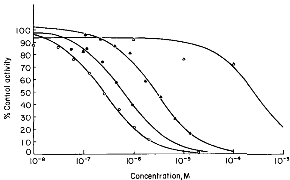
Figure 5. Inhibition of \text{Na}^+, \text{K}^+ -ATPase enzymatic activity by marinobufagin (O), marinobufotoxin (●), marinobufagin-3-sulfate (1a) (▲) and, 12 \beta -hydroxytetrahydroresibufogenin-3-sulfate (2) (Δ).
