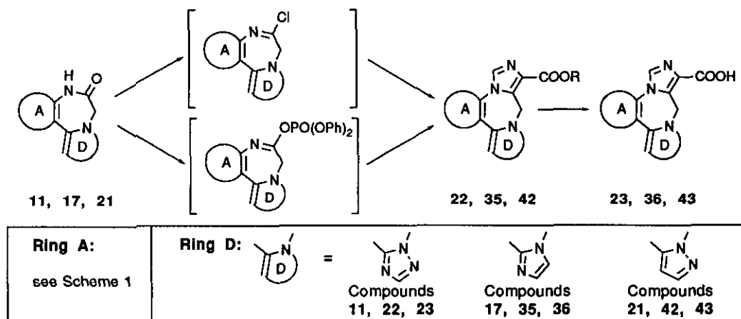
Scheme 2. Annelation of the tricyclic benzo- and thienodiazepinones (11, 17 and 21) with isocyanoacetic esters
