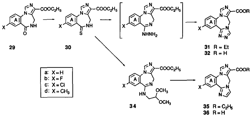
Scheme 3. Fusing a heterocyclic ring D (1,2,4-triazole or imidazole) on tricyclic imidazobenzodiazepinones (29)
