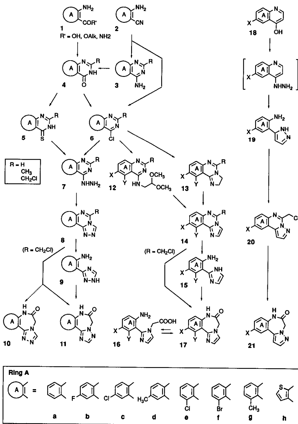
Scheme 1. Synthesis of the tricyclic benzo- and thienodiazepinones (11, 17 and 21)
