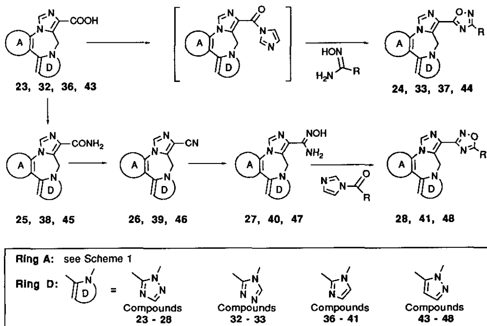
Scheme 4. Synthesis of the 5- and the 3-(1,2,4)-oxadiazolyl rings from carboxylic acids
