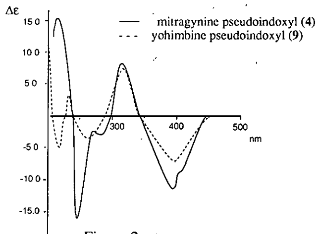
Figure 2 : CD Spectra of (4) and (9)
