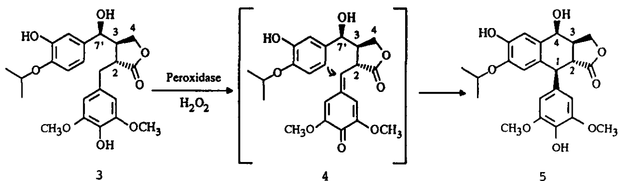
Scheme 1. Biotransformation of dibenzylbutanolide (3) to cyclic product (5) via hypothetical quinone methide intermediate (4) with peroxidase enzymes.
