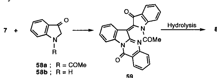
Scheme 19
