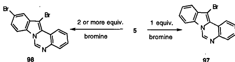
Scheme 34
