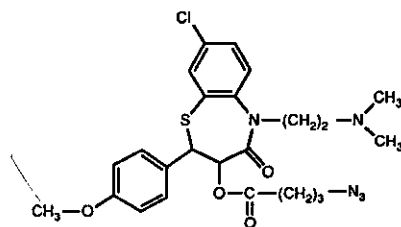
Azidobutyryl clemizem
