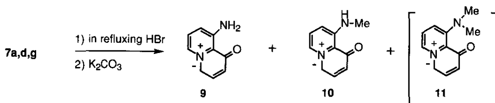
Scheme 6
