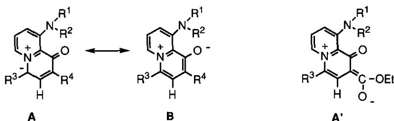
Scheme 7
