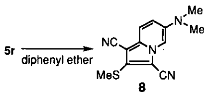
Scheme 5
