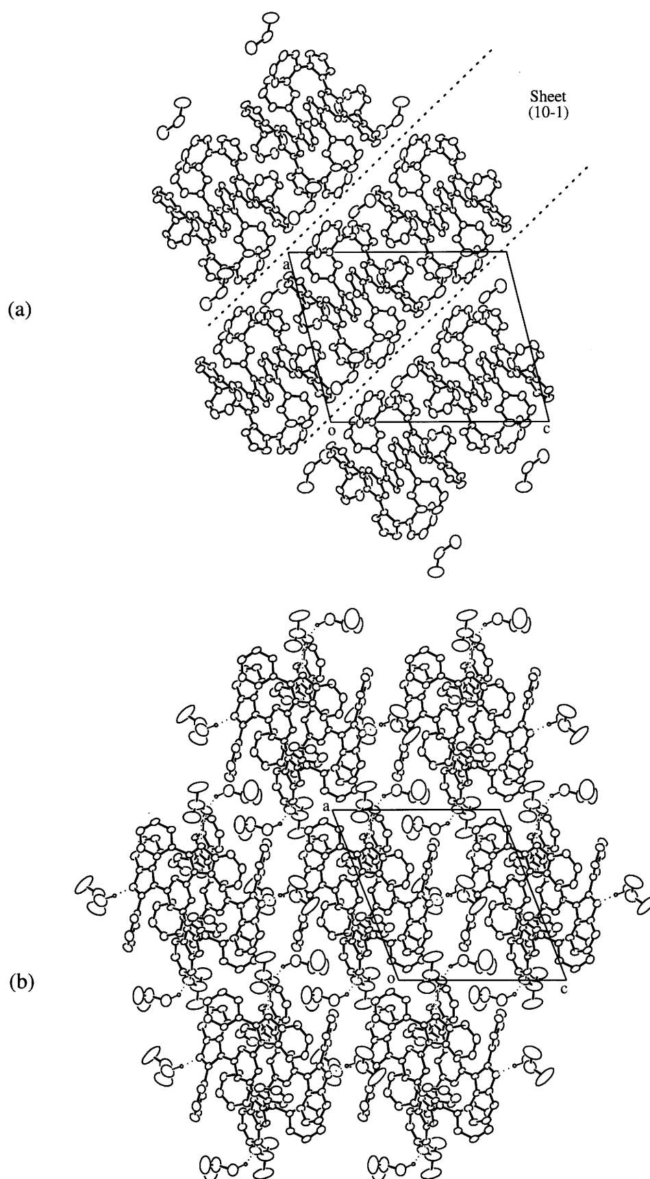
Figure 2. View of the packing of compounds (a) 6c and (b) 8c , both along the b axis and both showing the pseudo-hexagonal packing of rods parallel to that axis and centered at (3/4, 0, 1/4) and (1/2, 0, 0) . Hydrogen atoms have been omitted for more clarity.
