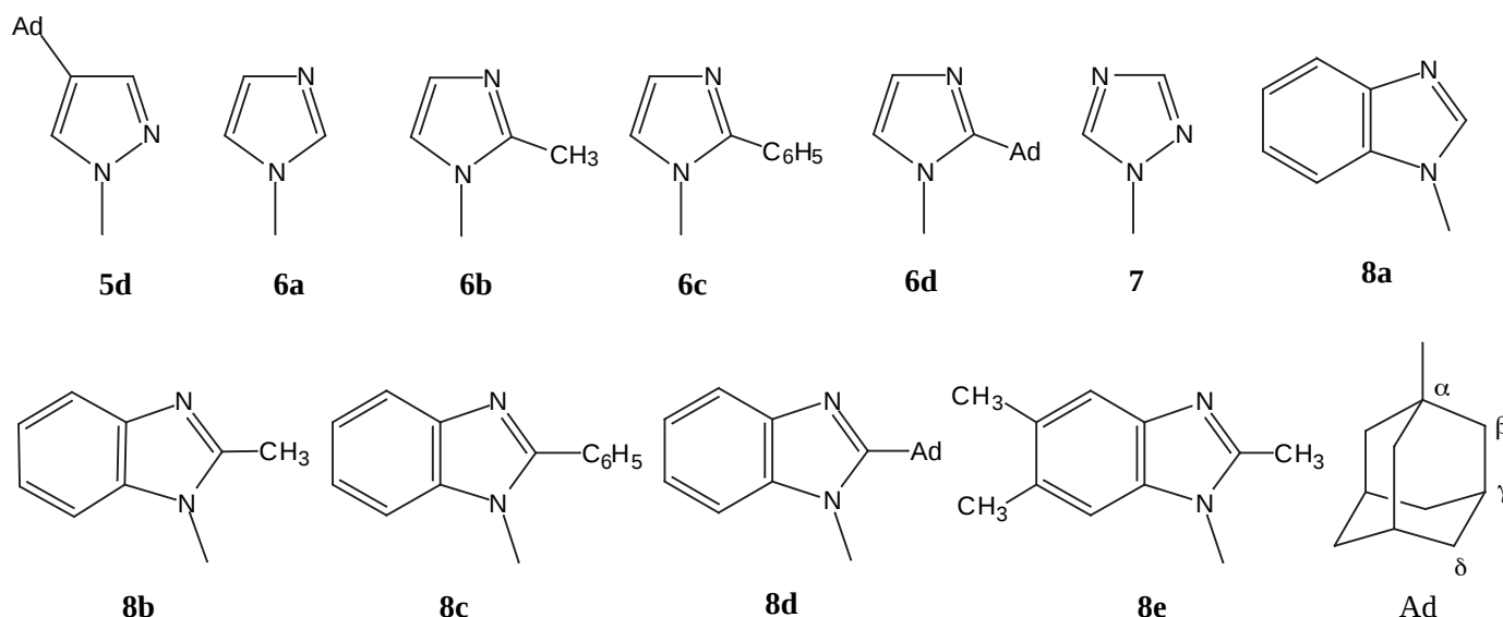
Scheme 1. The azol-1-yl substituents on 1,3,5-triazine ring. For the corresponding azoles, an H is added
