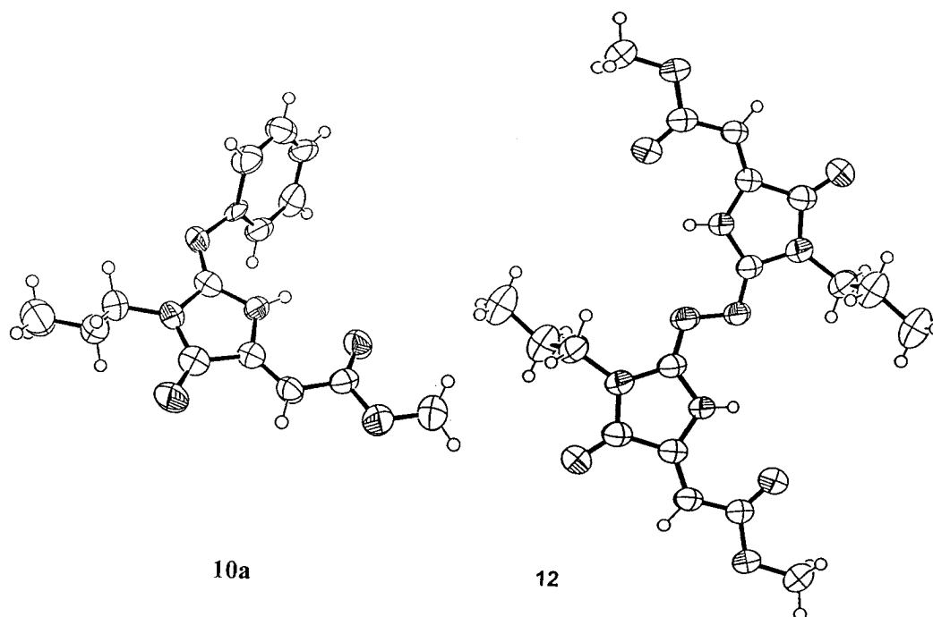
Figure 2. ORTEP view of compounds ( 10a ) and ( 12 )
