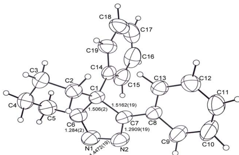
Figure 4. ORTEP plot of 3,3a-Diphenyl 4,5,6,7-tetrahydro-3a H -indazole ( 10c )
