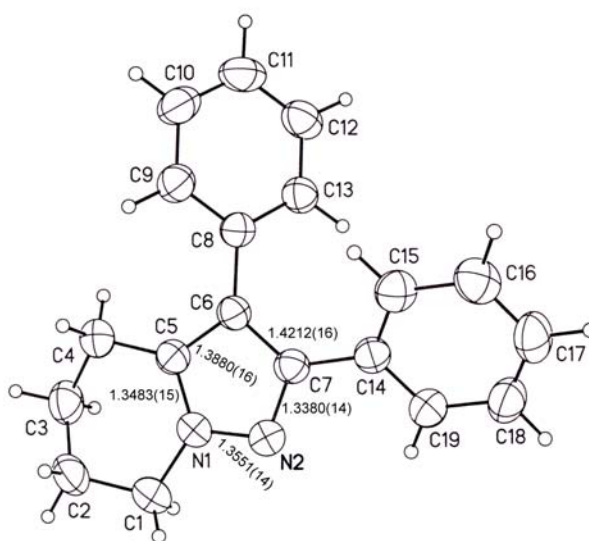
Figure 5. ORTEP plot of 2,3-Diphenyl 4,5,6,7-tetrahydropyrazolo[1,5- a ]pyridine ( 11c )
