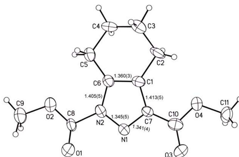
Figure 3. ORTEP Plots of Dimethyl 4,5,6,7- tetrahydro-indazole-1,3-dicarboxylate ( 12a )
