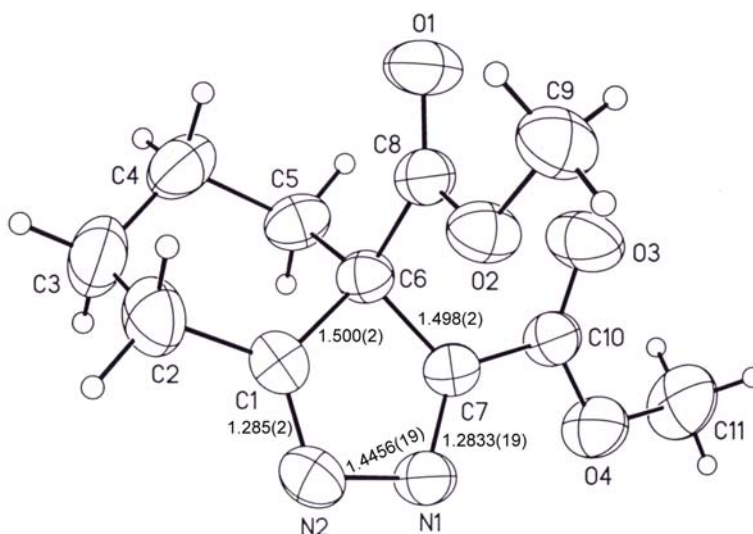
Figure 1. ORTEP Plots of Dimethyl 4,5,6,7-tetrahydro-3aH-indazole-3,3a-dicarboxylate ( 10a )
